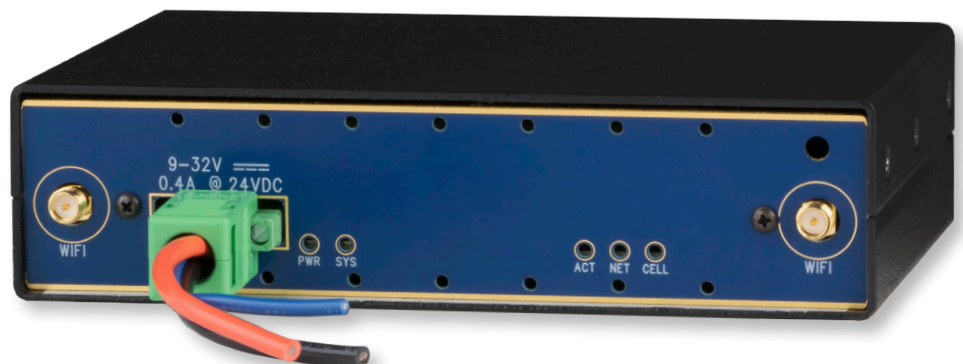
EN-2000™ Back Panel Pictured with Terminal Block Connector
