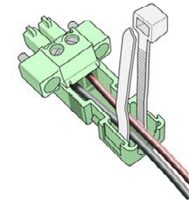
Cable-Tie through Bottom of DC Power Connector Shell
