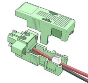
Top Section of Shell above Cabled Lower Shell Assembly
