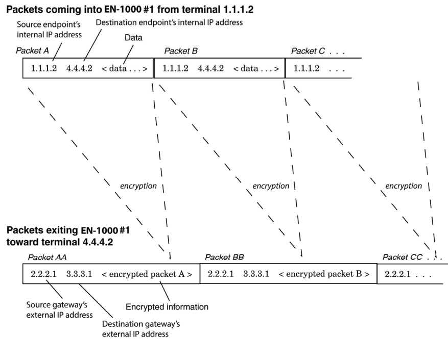
Figure D-2. Sample IPsec Encryption and Encapsulation
