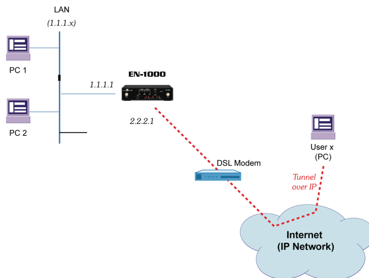
Figure D-3. EN-1000 Terminating Tunnel from VPN Client
