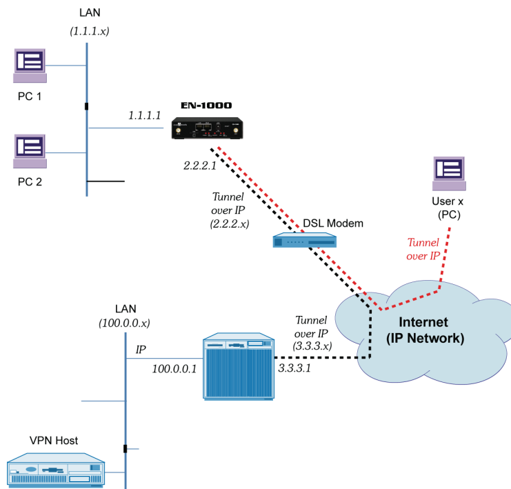
Figure D-4. EN-1000 Tunnel Switching between VPN Client and VPN Host
